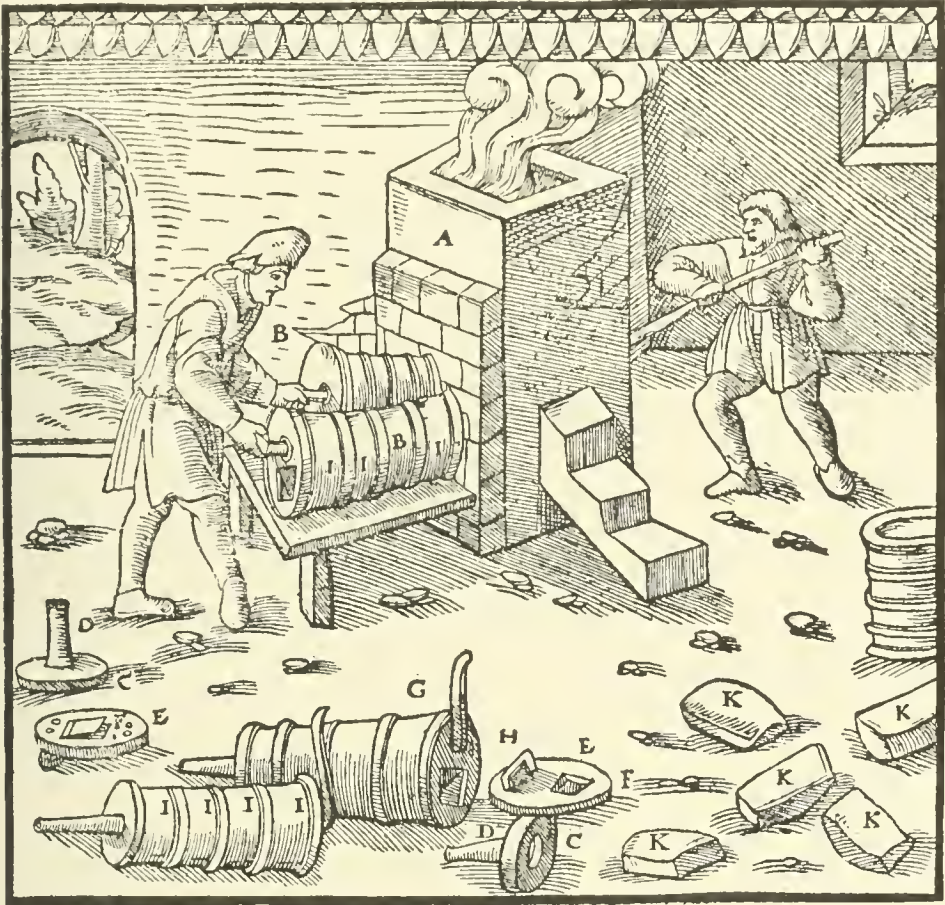
A—FURNACE. B—BELLOWS. C—IRON DISC. D—NOZZLE. E—WOODEN DISC. F—BLOW-HOLE. G—HANDLE. H—HAFT. I—HOOPS. K—MASSES OF TIN.
